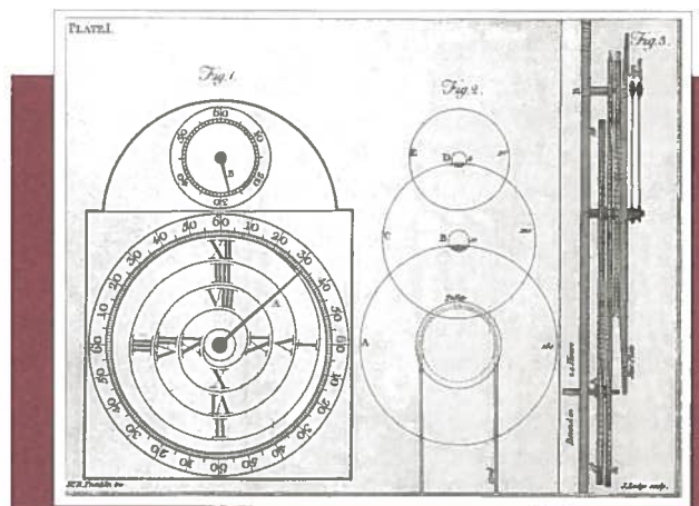
Benjamin Franklin’s three-wheel clock, in James Ferguson, Select Mechanical Exercises , 2d ed. (London, 1778).
